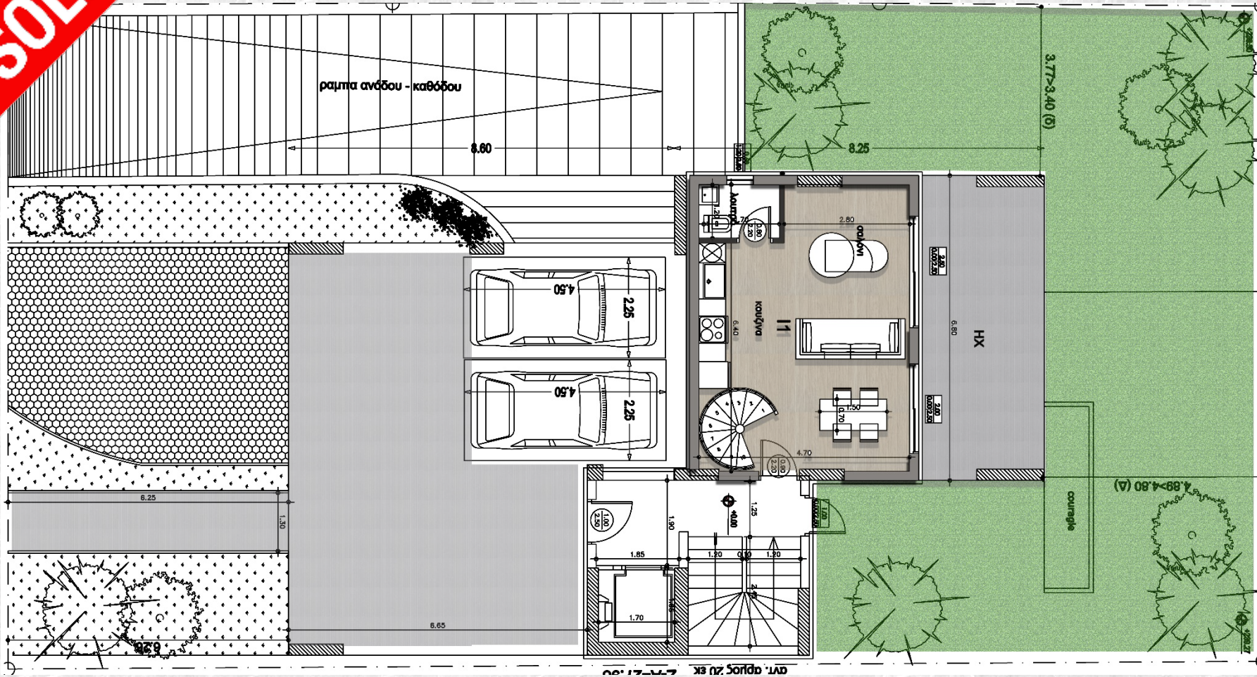
Maisonette of ground floor (Ground Floor Level)
